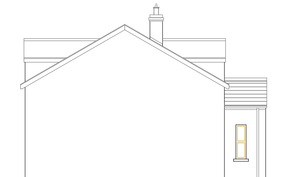
Proposed LHS Elevation -1:100-
