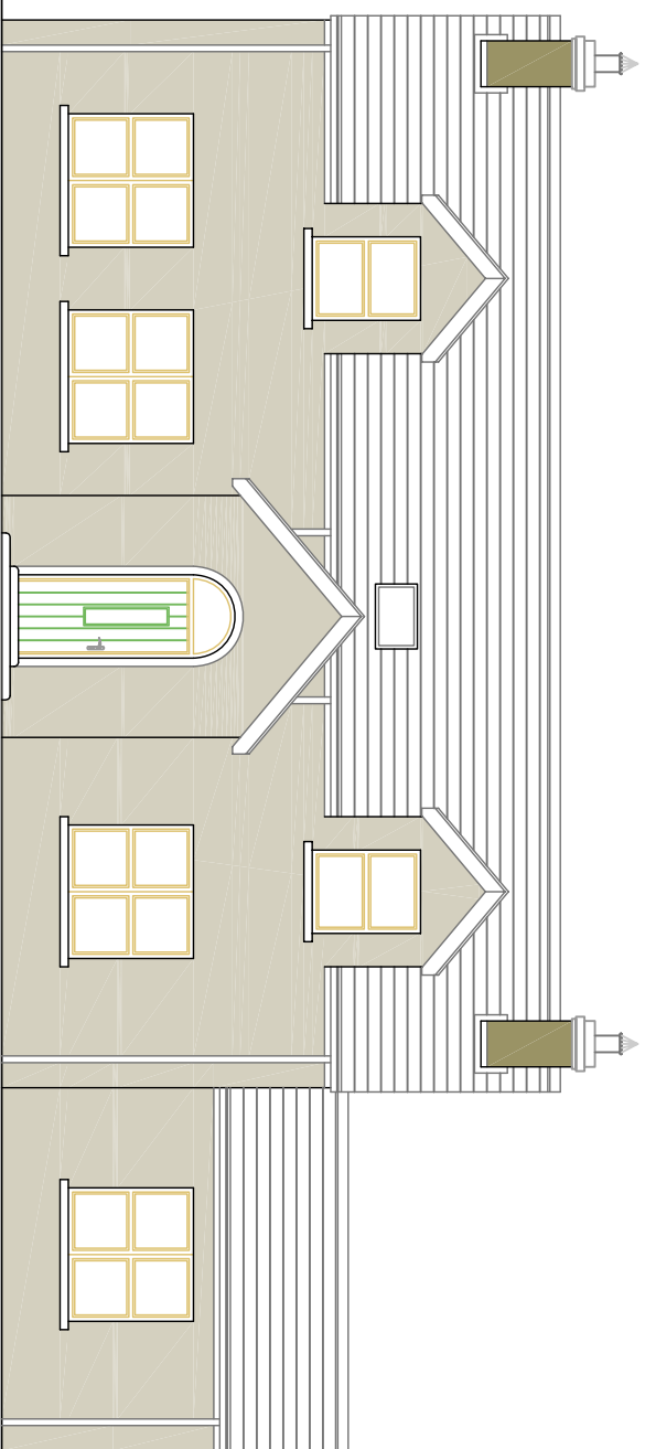
Proposed Front Elevation -1:100-
