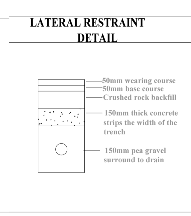
PROTECTION TO DRAINS
