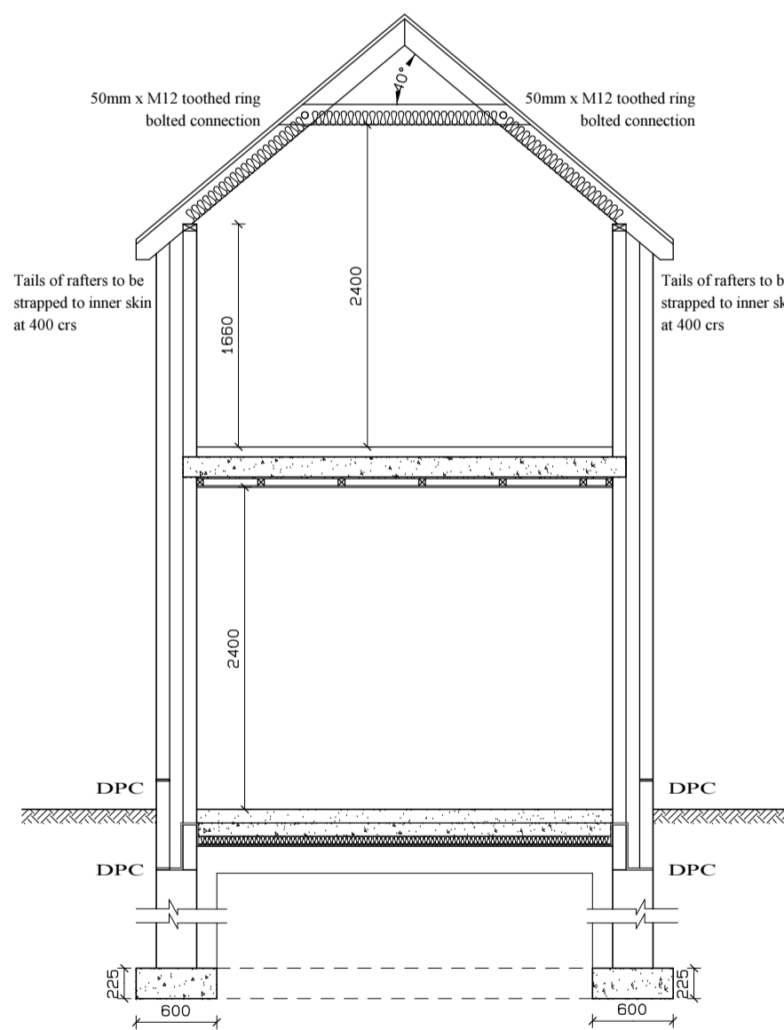
Section E-E
