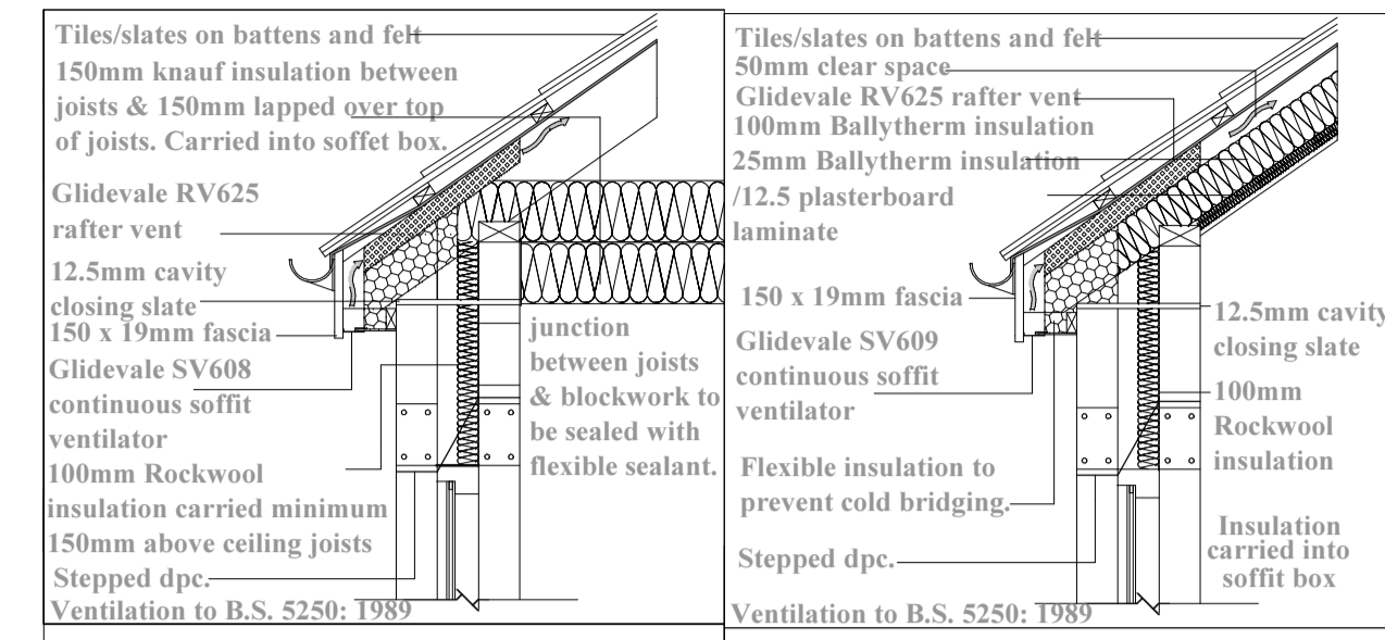
PORCH EAVES DETAIL
