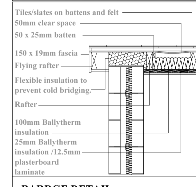
BARDGE DETAIL
