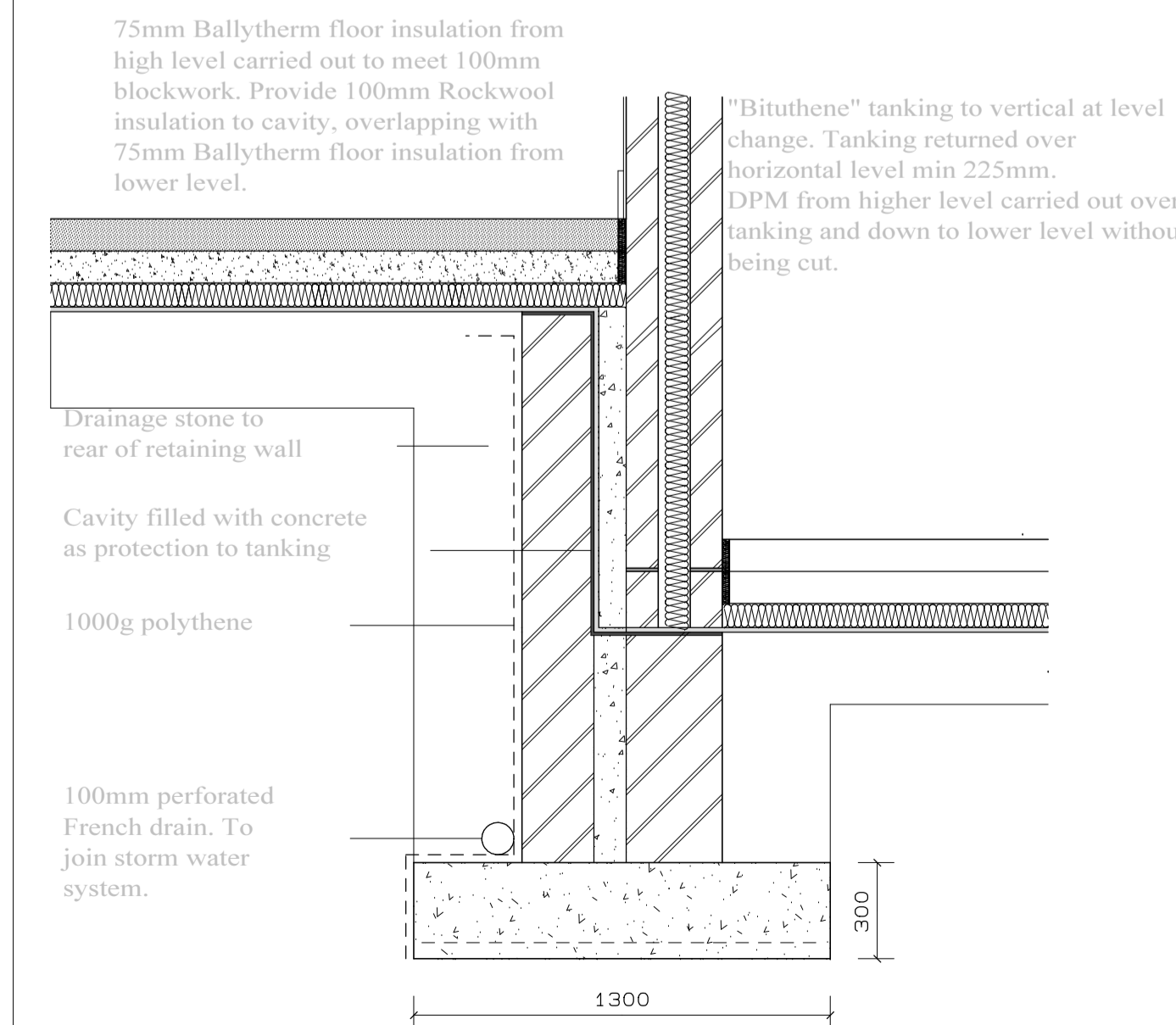
FLOOR INSULATION & DPM DETAIL
