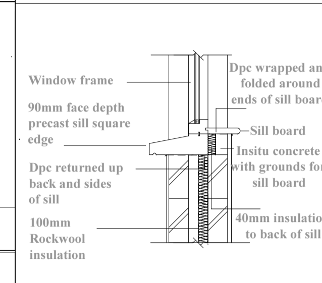
SILL DETAIL
