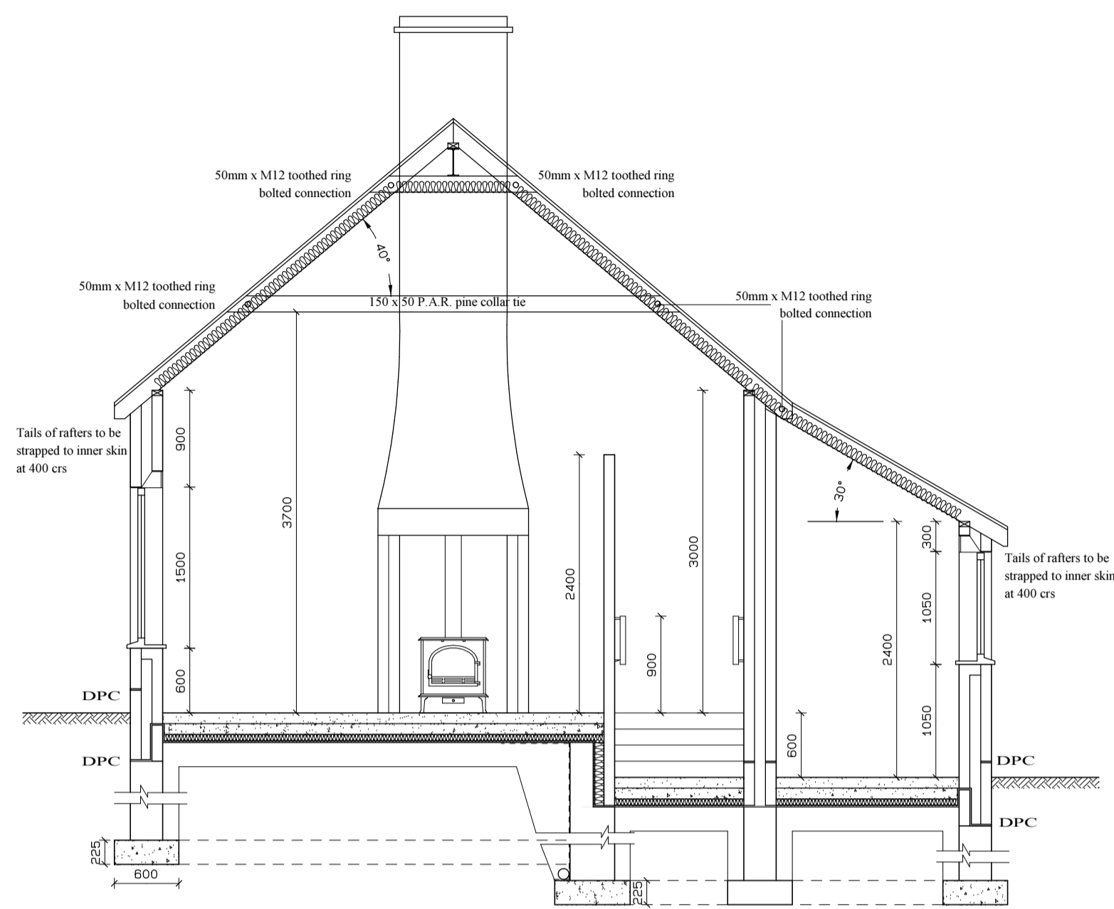
Section B-B
