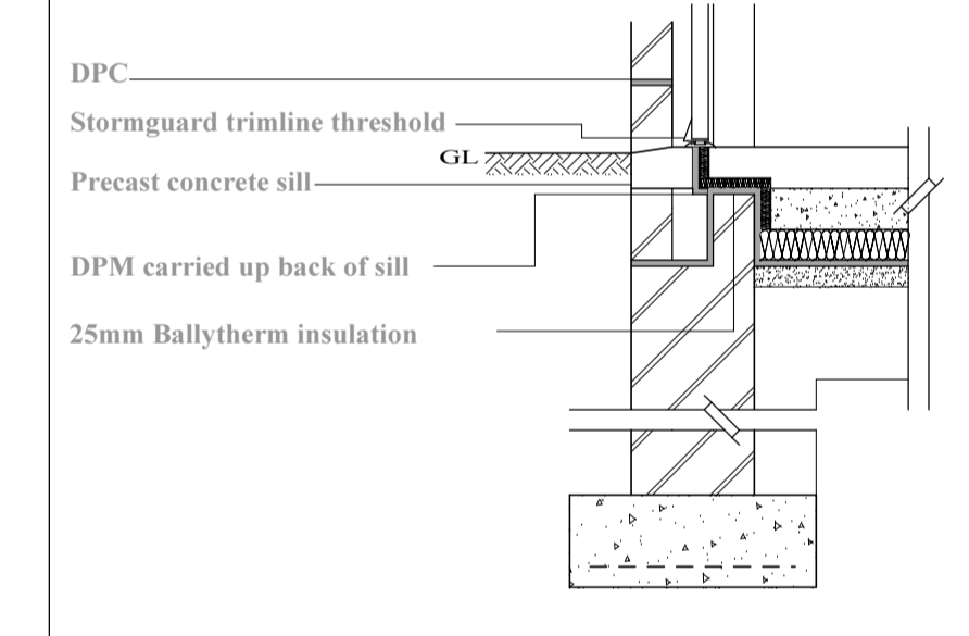
DPM DETAIL THRESHOLD DETAIL
