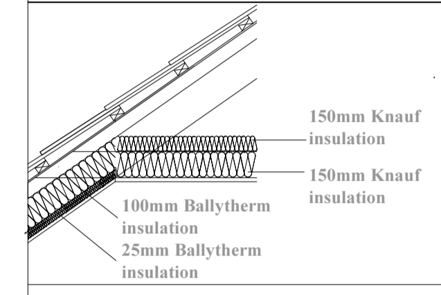
ROOF INSULATION
