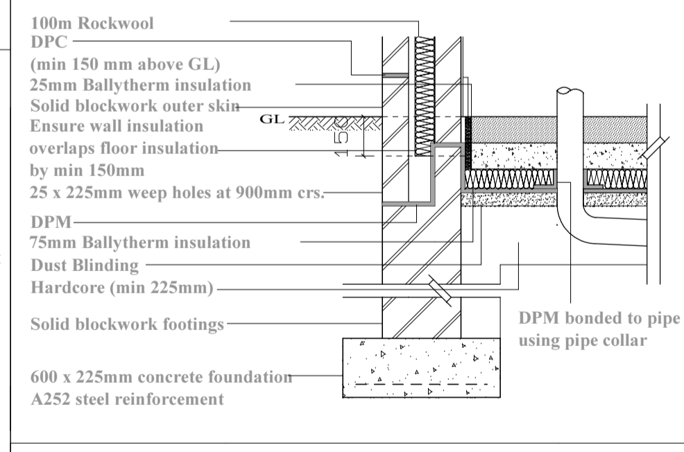
FLOOR INSULATION & DPM DETAIL
