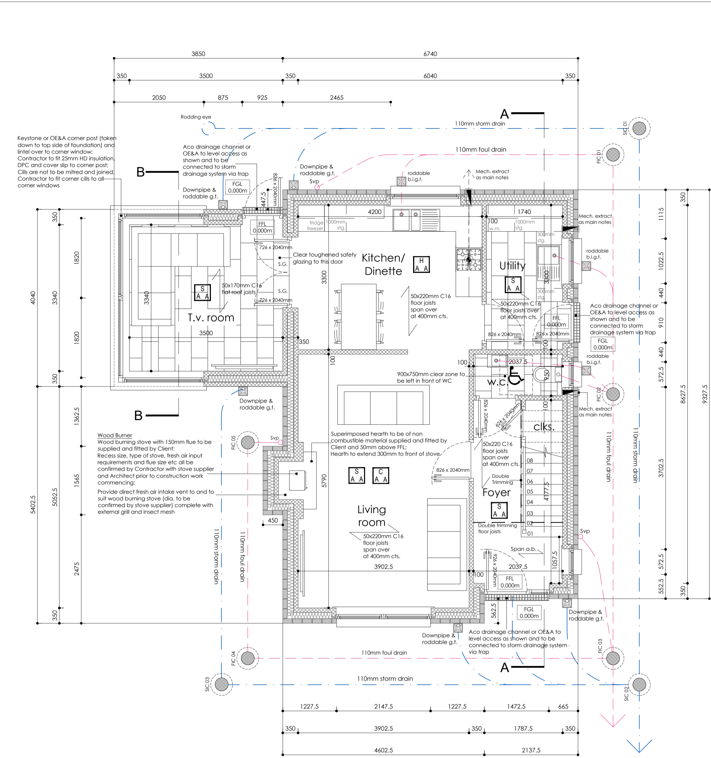
Proposed ground floor plan 67.16 m. sq.
